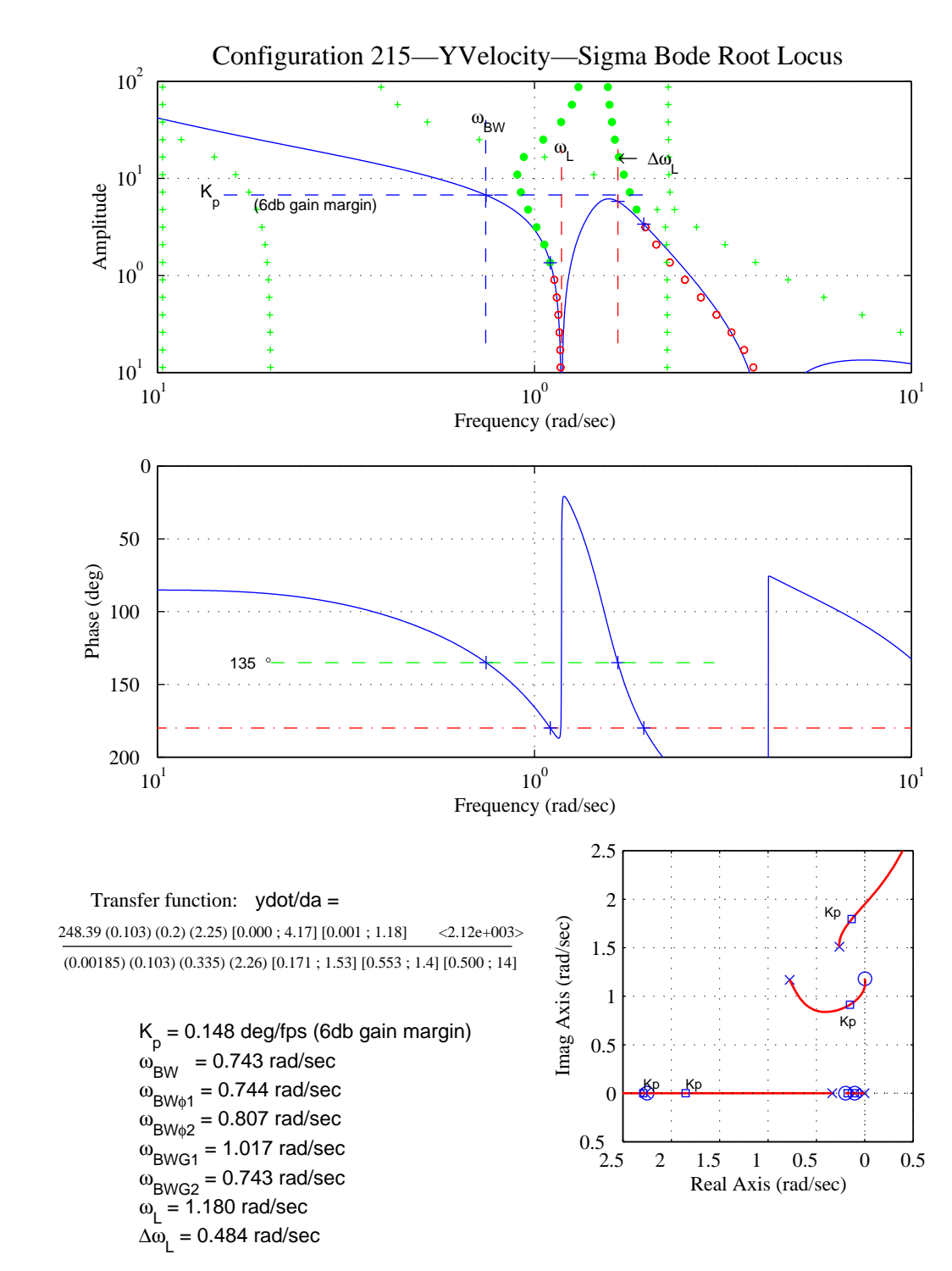
Figure D-46. Lateral Translational-Rate-Loop-Closure Characteristics – Configuration 215.
