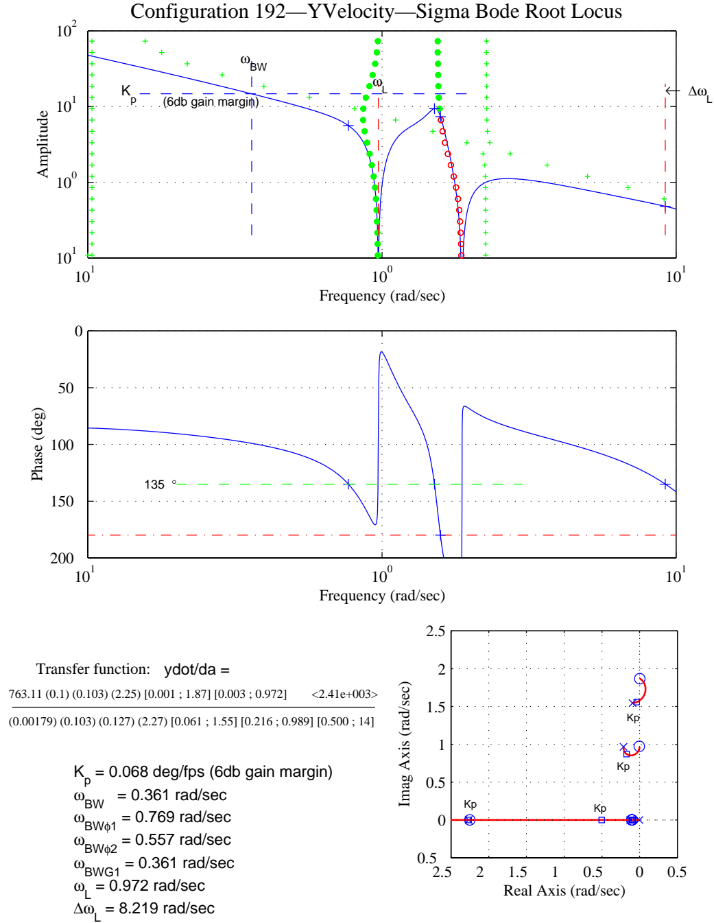
Figure D-41. Lateral Translational-Rate-Loop-Closure Characteristics – Configuration 192.
