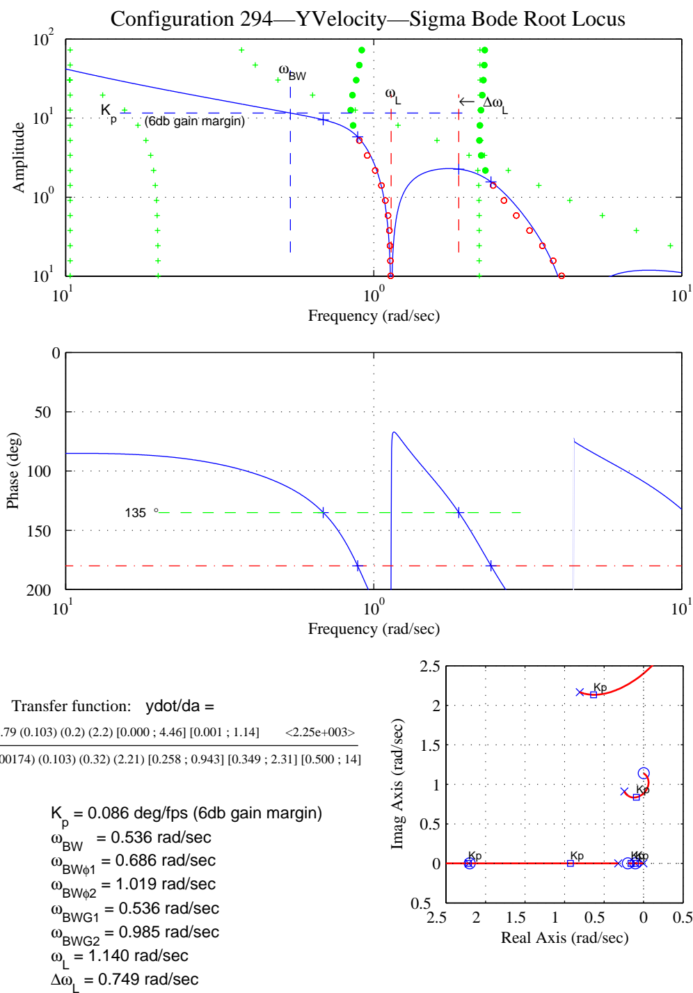
Figure D-53. Lateral Translational-Rate-Loop-Closure Characteristics – Configuration 294.
