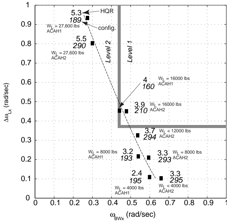
a) Effect of Load Mass Ratio - Longitudinal Axis
