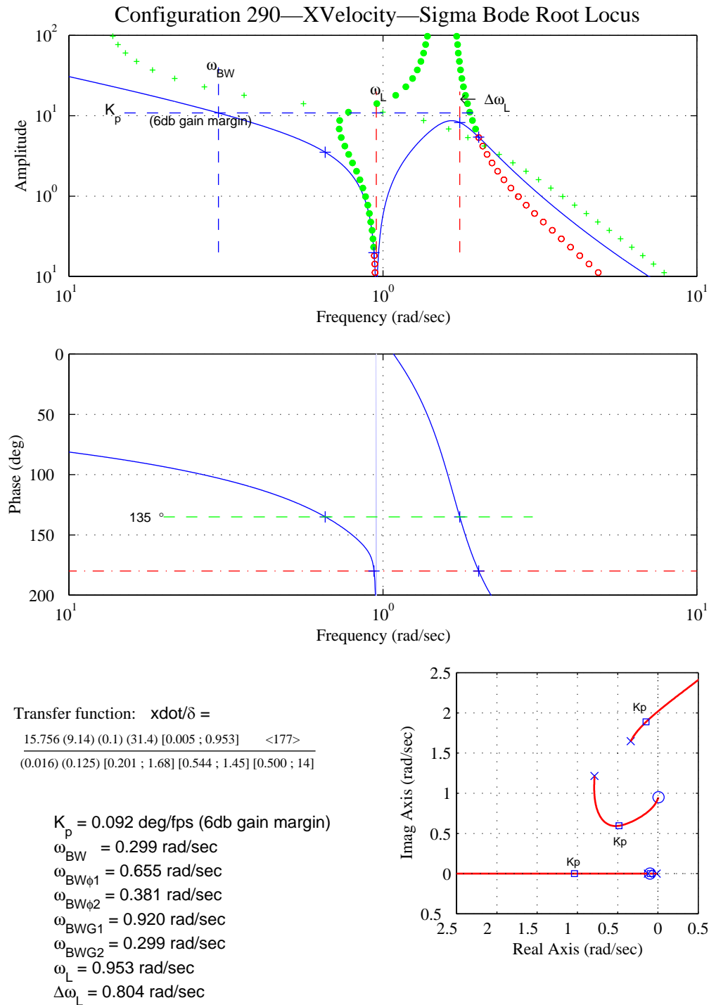
Figure D-24. Longitudinal Translational-Rate-Loop-Closure Characteristics – Configuration 290.
