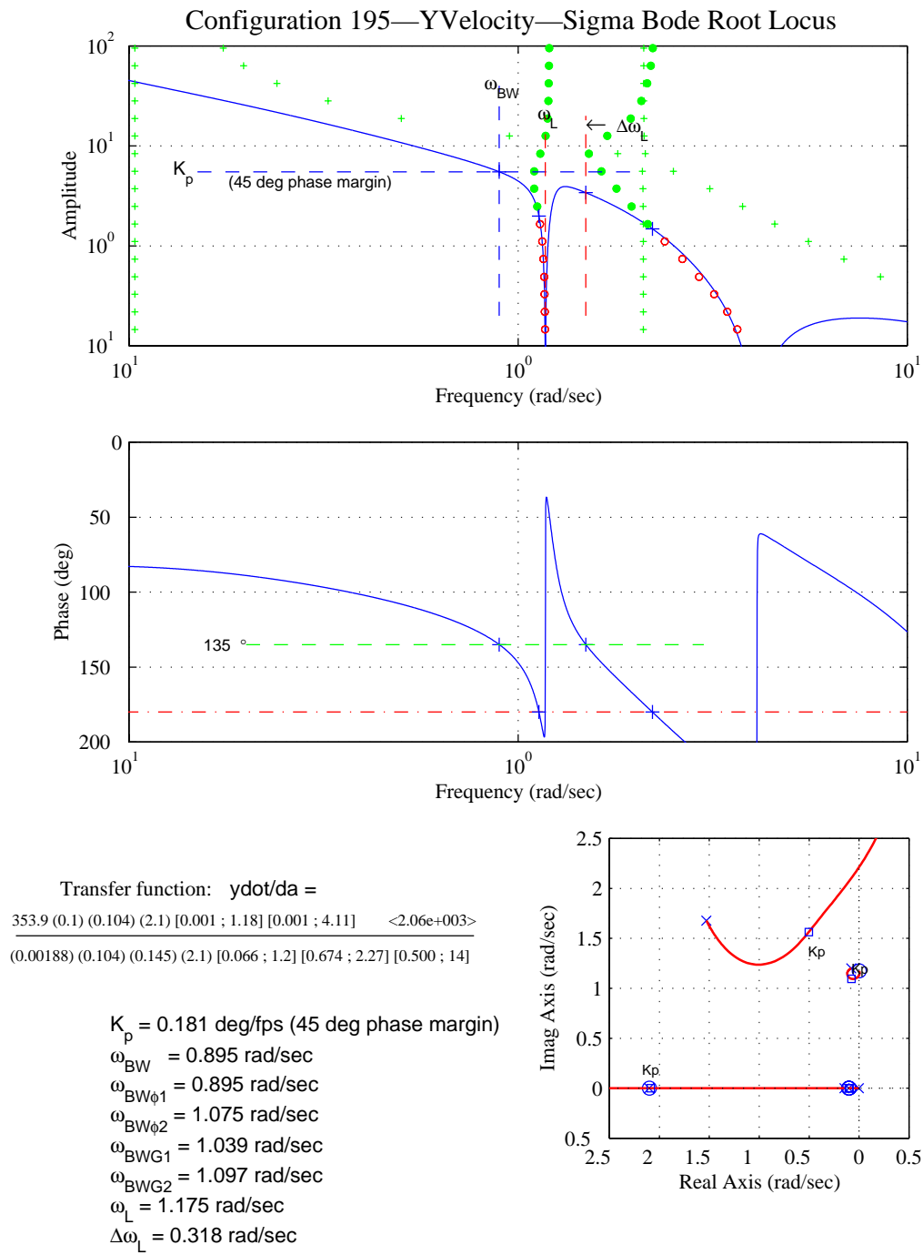
Figure D-43. Lateral Translational-Rate-Loop-Closure Characteristics – Configuration 195.
