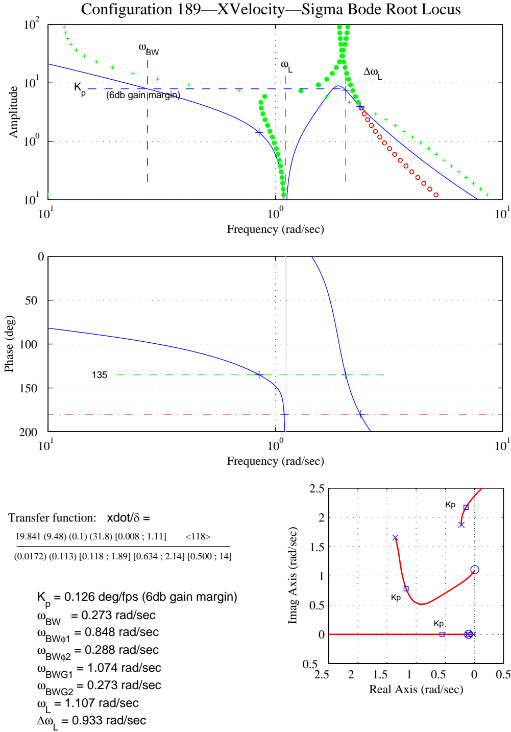
Figure D-13. Longitudinal Translational-Rate-Loop-Closure Characteristics – Configuration 189.
