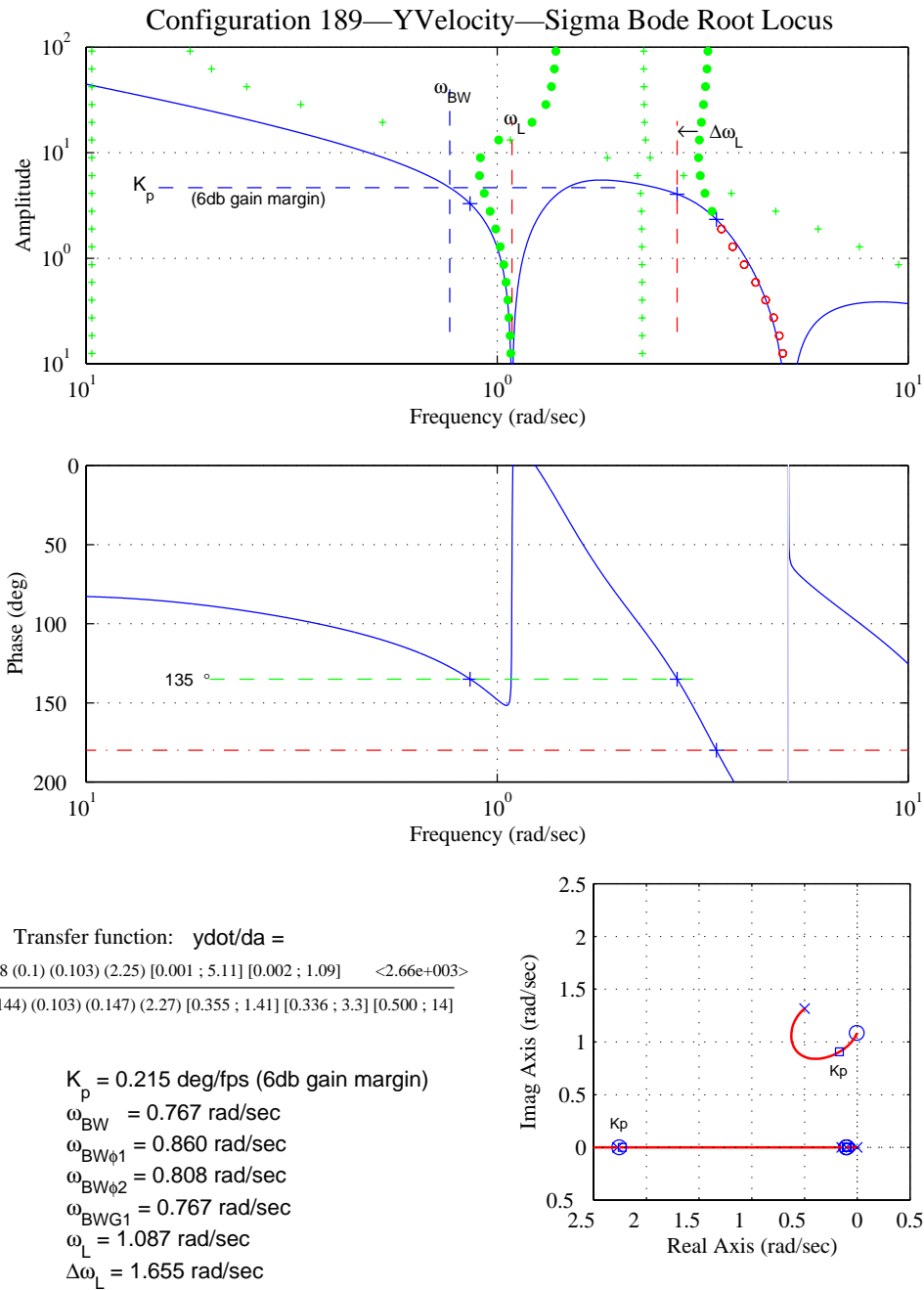
Figure D-39. Lateral Translational-Rate-Loop-Closure Characteristics – Configuration 189.
