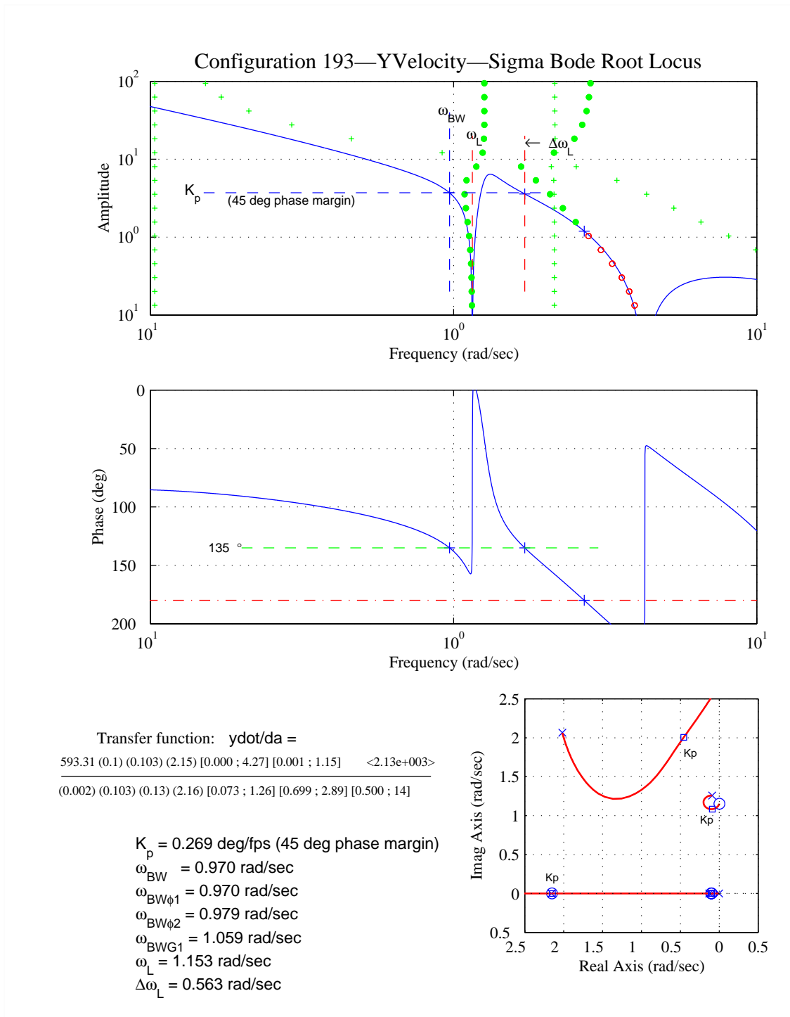
Figure D-42. Lateral Translational-Rate-Loop-Closure Characteristics – Configuration 193.
