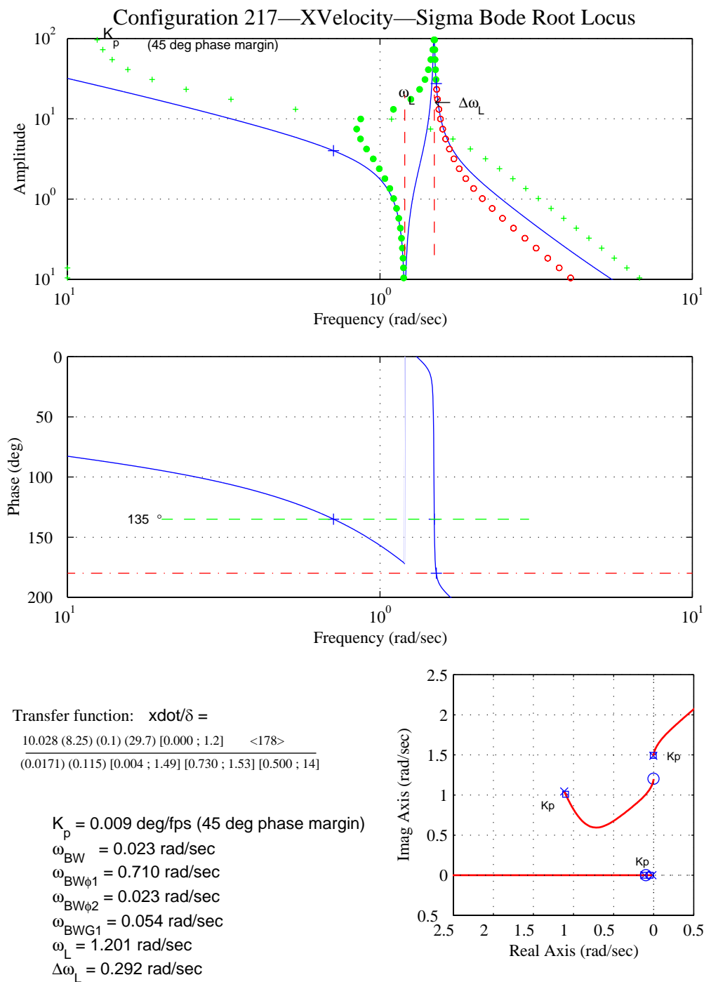
Figure D-20. Longitudinal Translational-Rate-Loop-Closure Characteristics – Configuration 217.
