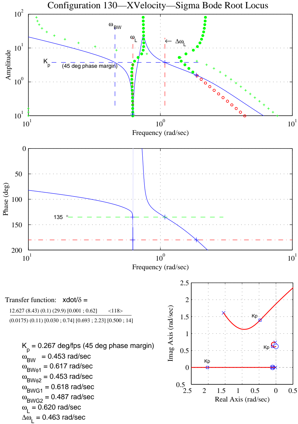
Figure D-5. Longitudinal Translational-Rate-Loop-Closure Characteristics – Configuration 130.
