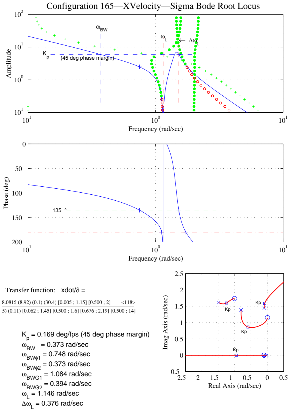
Figure D-12. Longitudinal Translational-Rate-Loop-Closure Characteristics – Configuration 166.
