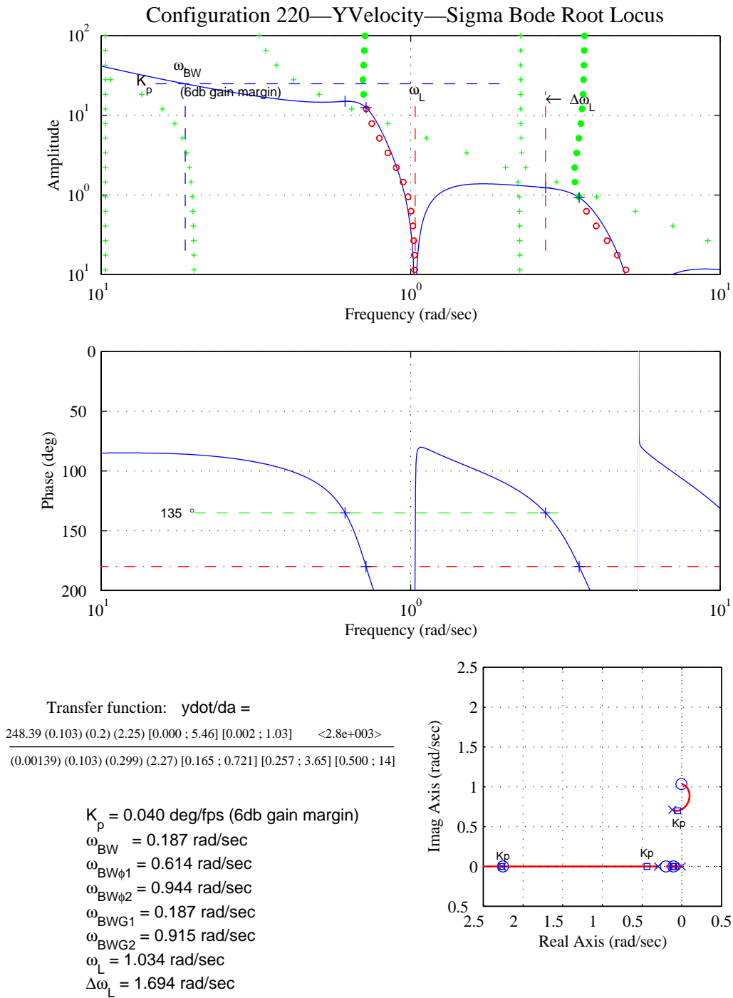
Figure D-48. Lateral Translational-Rate-Loop-Closure Characteristics – Configuration 220.
