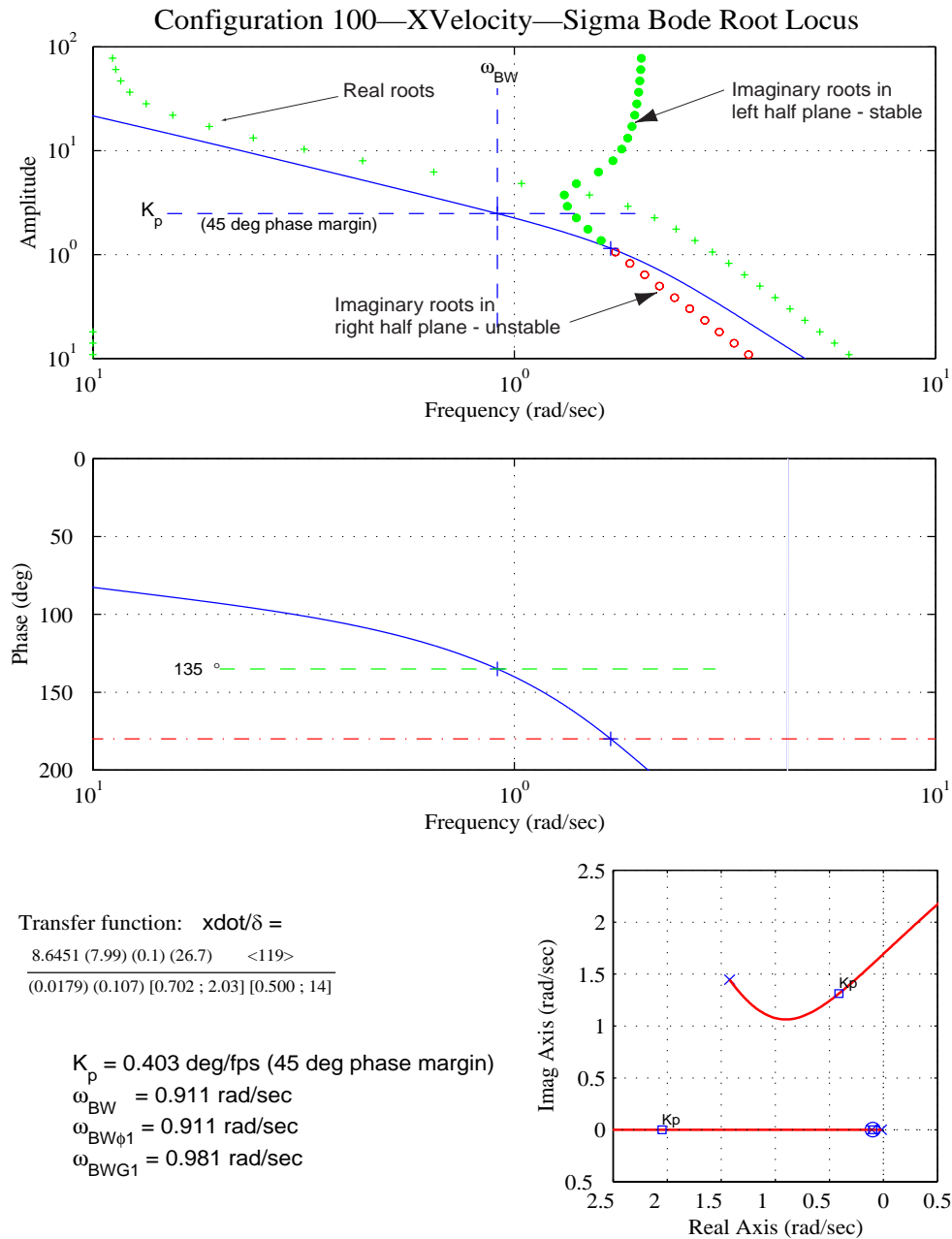
Figure D-1. Longitudinal Translational-Loop-Closure Characteristics – Configuration 100 – Load Off.
