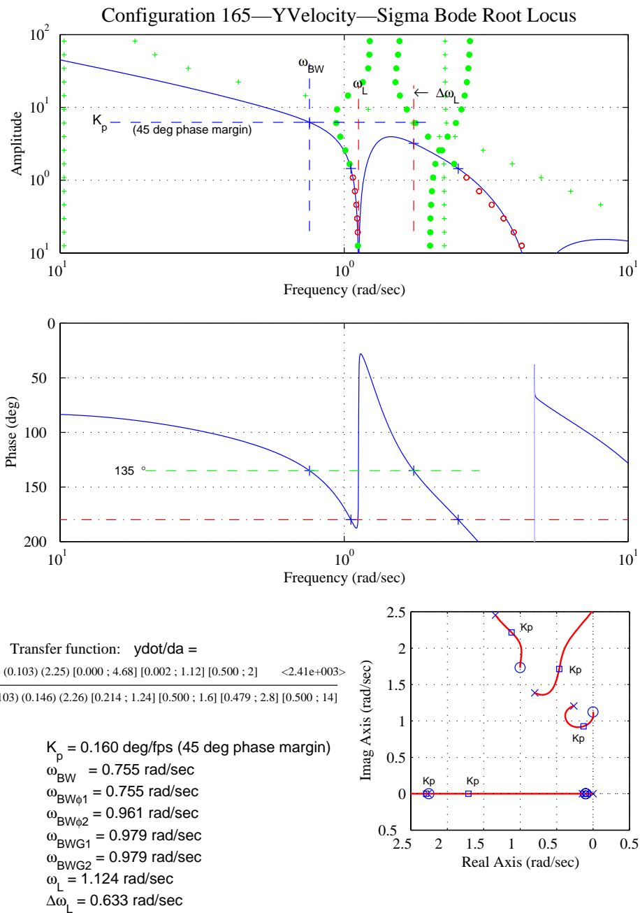
Figure D-37. Lateral Translational-Rate-Loop-Closure Characteristics – Configuration 165.
