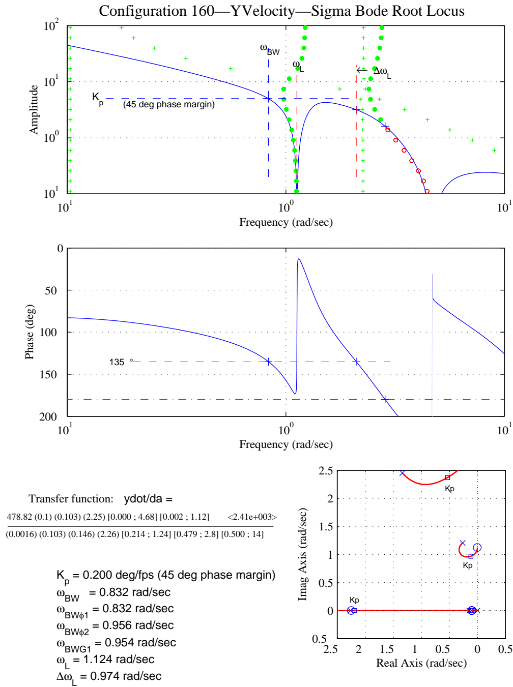
Figure D-36. Lateral Translational-Rate-Loop-Closure Characteristics – Configuration 160.
