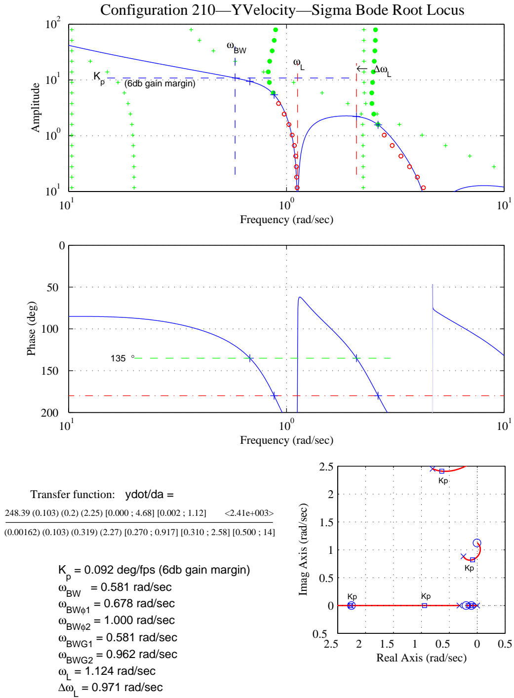
Figure D-44. Lateral Translational-Rate-Loop-Closure Characteristics – Configuration 210.
