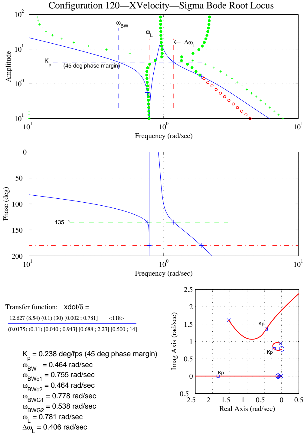
Figure D-4. Longitudinal Translational-Rate-Loop-Closure Characteristics – Configuration 120.
