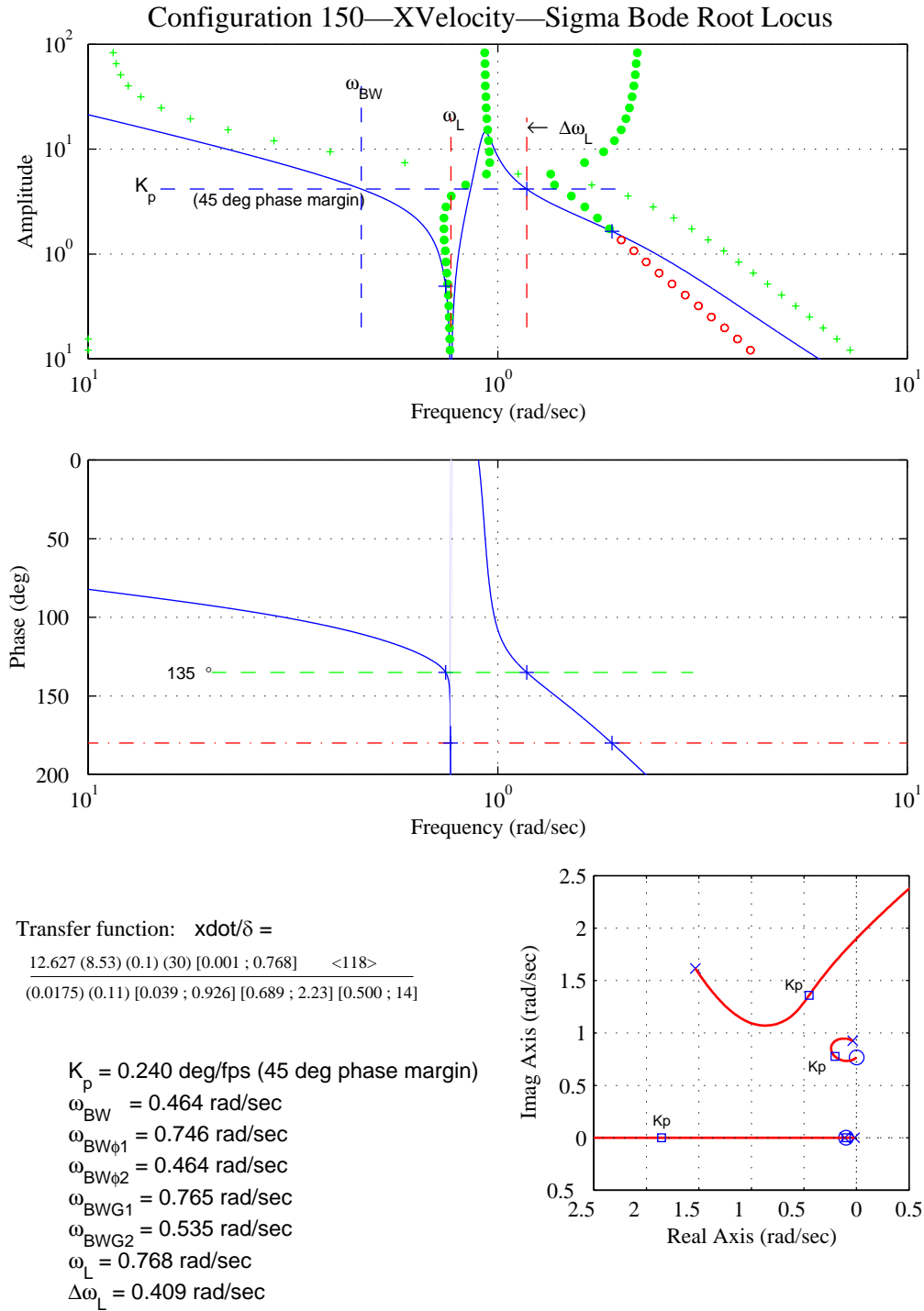
Figure D-7. Longitudinal Translational-Rate-Loop-Closure Characteristics – Configuration 150.
