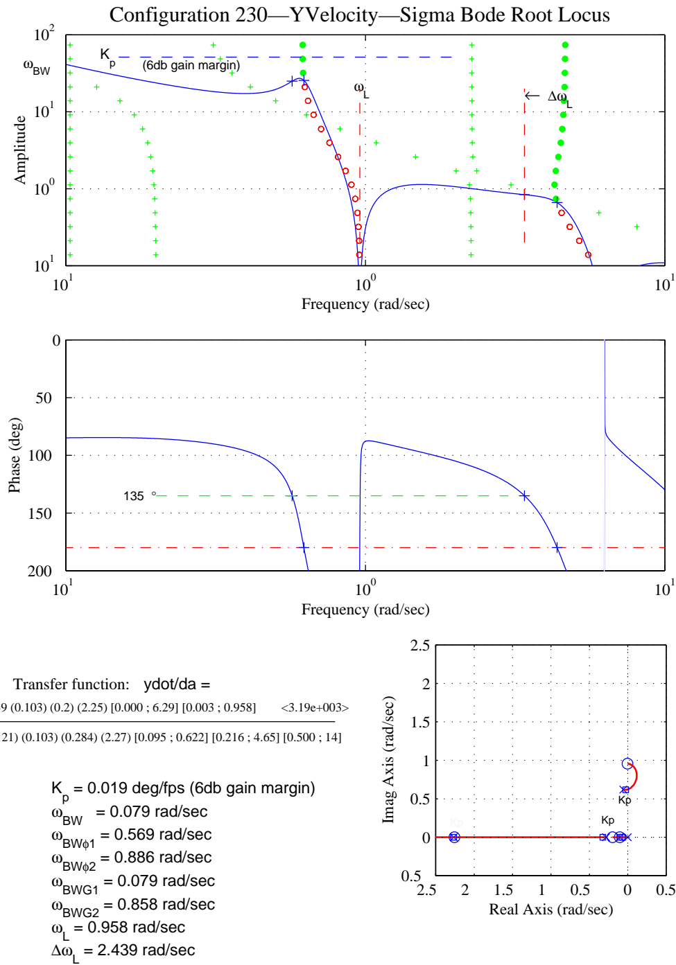
Figure D-49. Lateral Translational-Rate-Loop-Closure Characteristics – Configuration 230.
