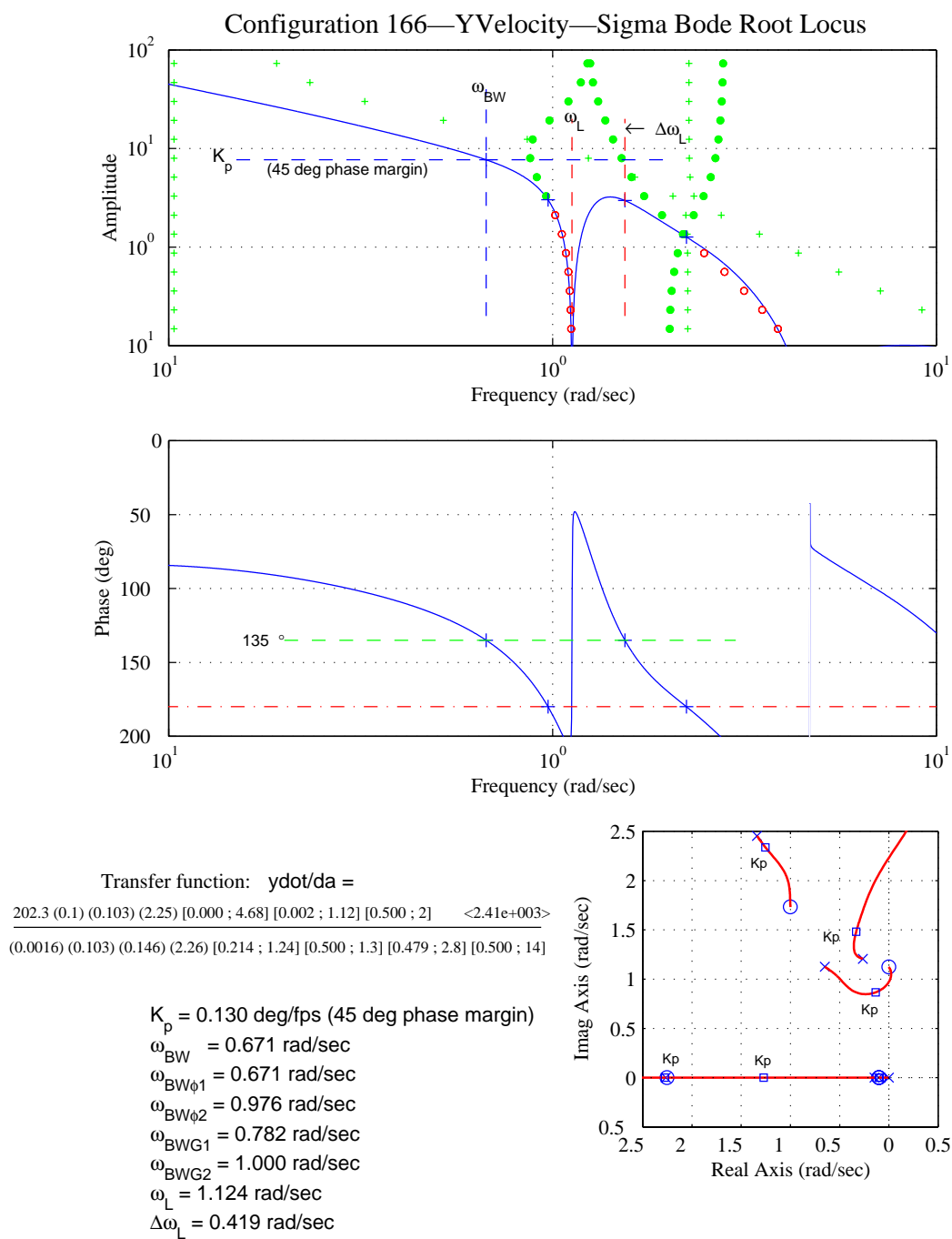
Figure D-38. Lateral Translational-Rate-Loop-Closure Characteristics – Configuration 166.
