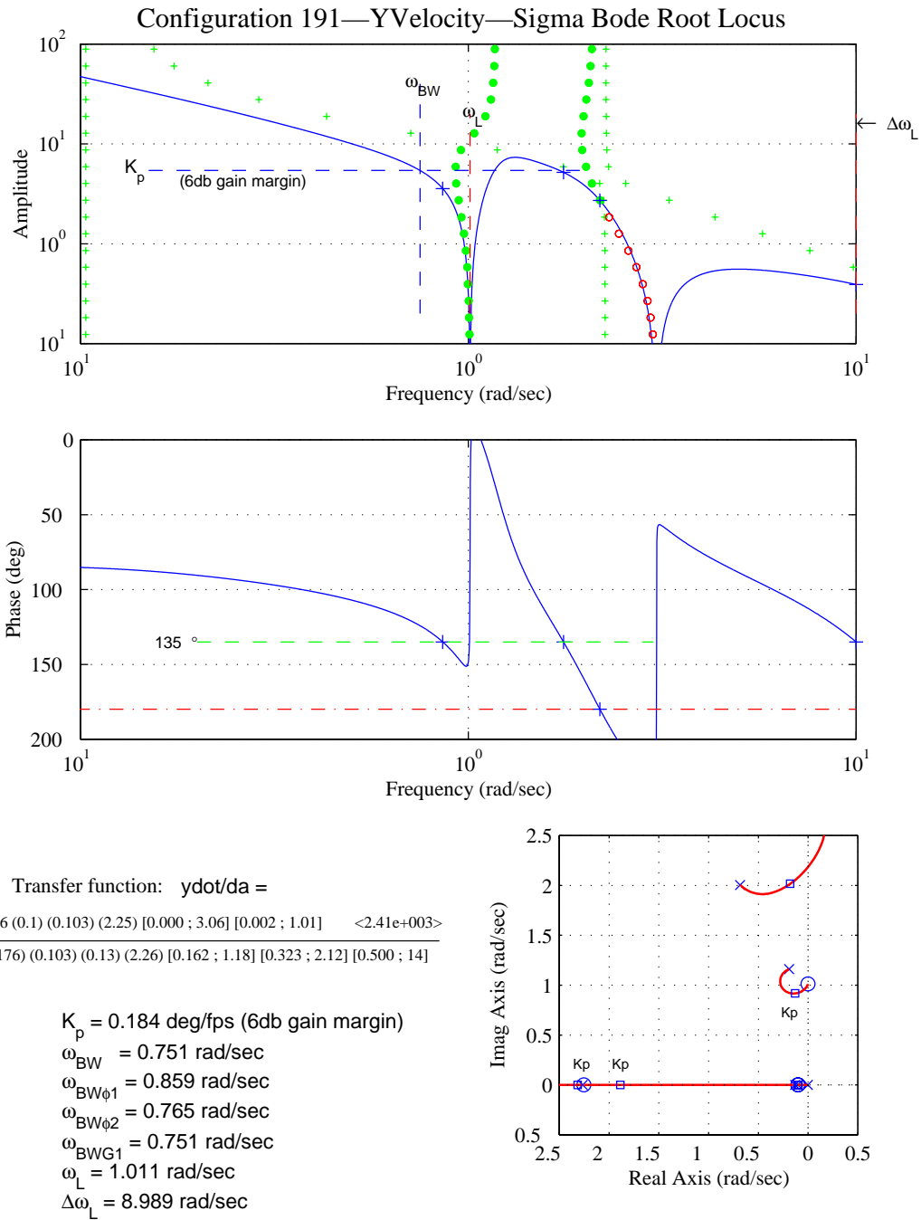
Figure D-40. Lateral Translational-Rate-Loop-Closure Characteristics – Configuration 191.
