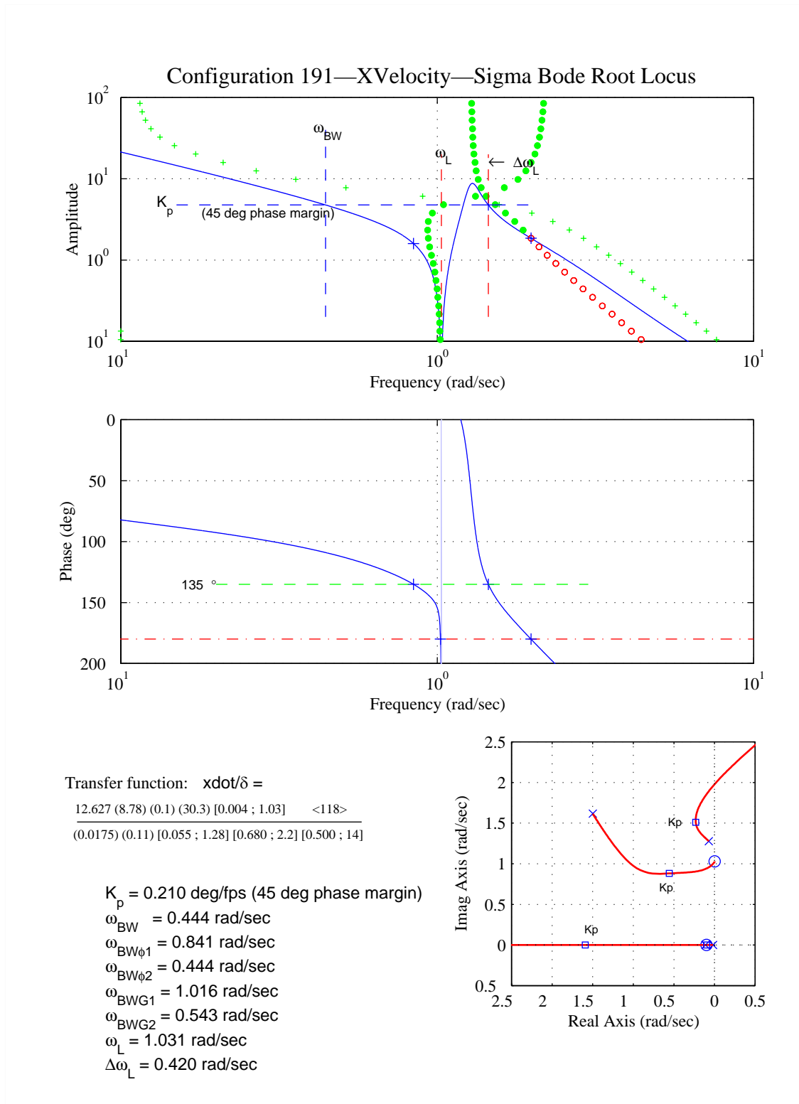
Figure D-14. Longitudinal Translational-Rate-Loop-Closure Characteristics – Configuration 191.
